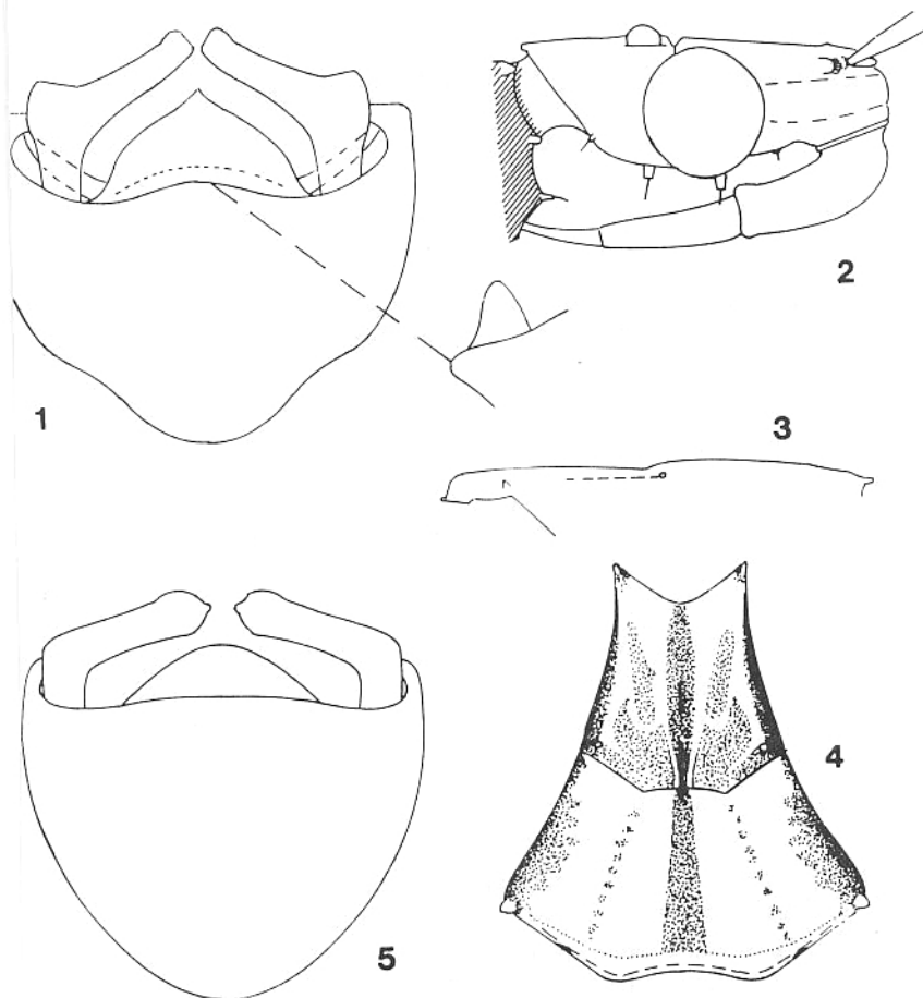
PLATE I.— Apronius octonotatus Champion, male, fig. 1. genital capsule, caudal view. Apronius planus n. sp., male; fig. 2. head, lateral; fig. 3. upper surface of pronotum, anterior end to the right, lateral; fig. 4. pronotum, dorsal; fig. 5. genital capsule.
