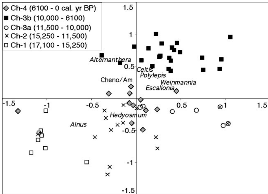
Figure 4 Results of a non-metric multivariate scaling (NMS) analysis, Axes 1 versus 2, for the samples ordination of selected fossil pollen taxa (pollen types shown in Fig. 5) from Laguna de Chochos, Peru. Samples are divided into their respective zones based on sedimentary characteristics. Samples with a cross superimposed on a circle with an asterisk are 'misplaced samples' placed at the upper limit of one zone, but whose NMS placement suggests affinity with the immediately overlying zone. Species that characterised these axes are shown by their relative placement
