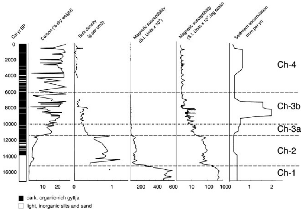
Figure 3 Physical characteristics of the core recovered from Lagune de Chochos, Peru, showing stratigraphy, percentage carbon, bulk density, magnetic susceptibility (ordinal and log-scaled), rates of sedimentation, and the zonation
