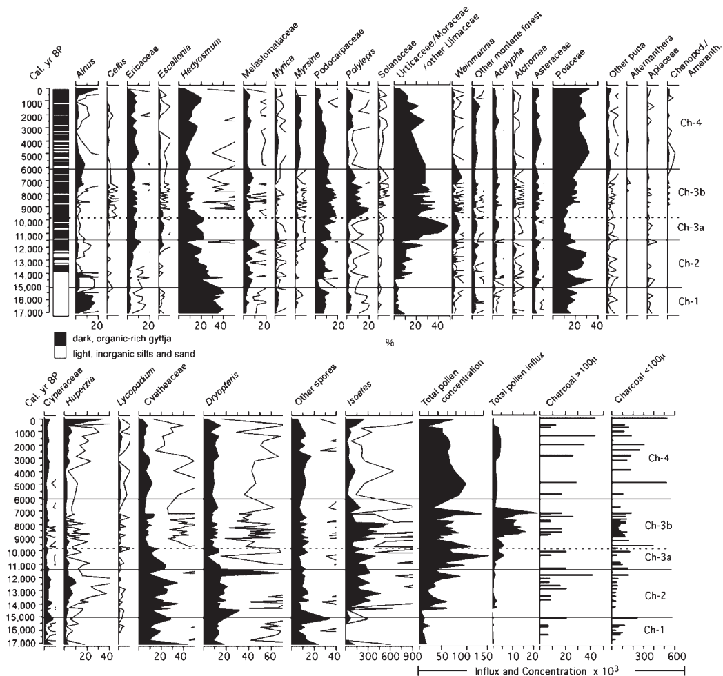
Figure 5 Selected fossil pollen and spores taxa and charcoal data from Laguna de Chochos. Note the x-axis scale for Isoetes has a more compressed scale than other taxa. Urticaceae/Moraceae/Ulmaceae are expressed as a percentage of the total terrestrial pollen sum, all other taxa are expressed as a percentage excluding Urticaceae/Moraceae/Ulmaceae
