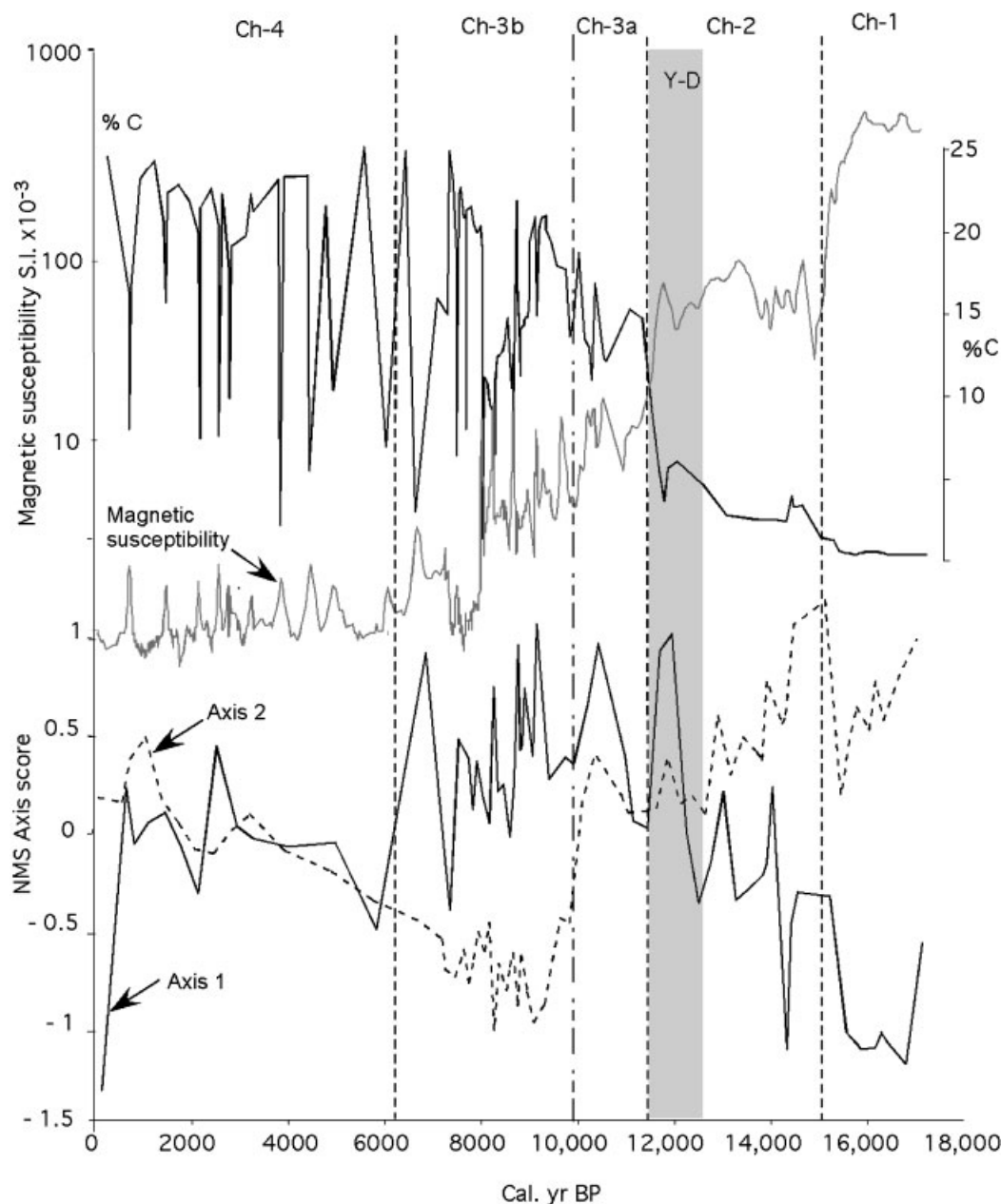
Figure 7 Synthesis of data from Laguna de Chochos showing the temporal variability of magnetic susceptibility, percentage carbon content, and NMS Axes 1 and 2 sample scores plotted against time. Vertical lines depict the zonation of the record and the shaded area represents the Younger Dryas period (12 600–11 500 cal. yr BP)
